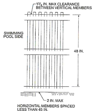
Detail 1. Figure AG-105.2(2) Private Swimming Pool Barrier Construction
